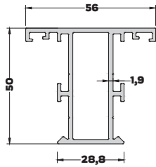
AB-6542 (1,125 kg/mt) ORTA KAYIT PROFİLİ
