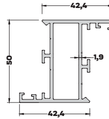
AB-6544 (1,125 kg/mt) Z KASA PROFİLİ
