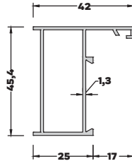
AL-223 (0,584 kg/mt) DAR KASA PROFİLİ
