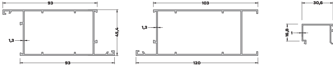
AL-3045 (1,088 kg/mt) KAPI KANAT PROFİLİ
