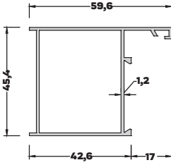
AL-3073 (0,548 kg/mt) GENİŞ KASA PROFİLİ
