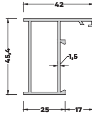
AL-246 (0,663 kg/mt) DAR KASA PROFİLİ
