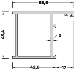
AL-208 (1,051 kg/mt) GENİŞ KASA PROFİLİ
