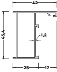
AL-3080 (0,548 kg/mt) DAR KASA PROFİLİ
