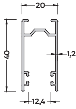
P-4067 (0,652 kg/mt) PANJUR YAN KASA PROFİLİ
