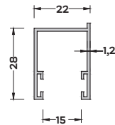
P-4062 (1,215 kg/mt) PANJUR YAN KASA PROFİLİ
