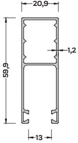
P-3947 (0,560 kg/mt) PANJUR YAN KASA PROFİLİ
