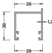
P-5040 (1,220 kg/mt) PANJUR YAN KASA PROFİLİ
