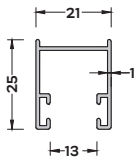
P-3416 (3,994 kg/mt) PANJUR YAN KASA PROFİLİ
