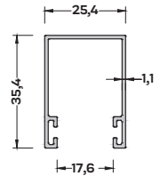
P-8482 (1,315 kg/mt) PANJUR YAN KASA PROFİLİ
