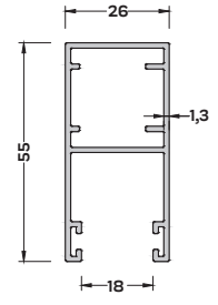
P-3457 (0,662 kg/mt) PANJUR YAN KASA PROFİLİ
