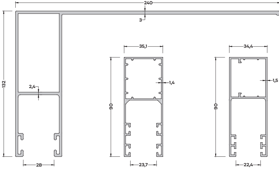
P-3416 (3,994 kg/mt) PANJUR YAN KASA PROFİLİ
