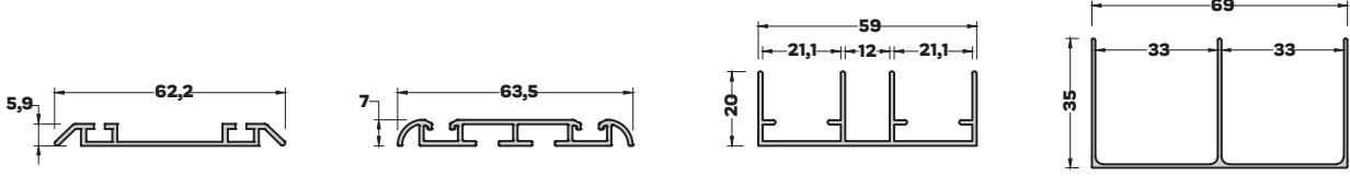
MB-5050 (0,309 kg/mt) ALT RAY PROFİLİ
