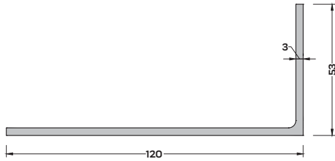
CK-4294 (1,387 kg/mt) L ANKRAJ PROFİLİ
