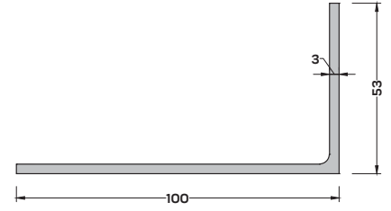
CK-4296 (1,224 kg/mt) L ANKRAJ PROFİLİ
