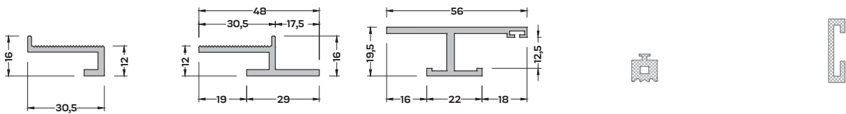
CK-6750 (0,328 kg/mt) ALT ASKI PROFİLİ
