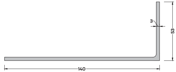
CK-4295 (1,549 kg/mt) L ANKRAJ PROFİLİ
