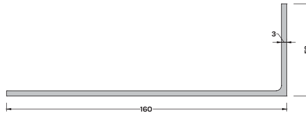
CK-4293 (1,712 kg/mt) L ANKRAJ PROFİLİ
