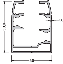
900-1102 (1,436 kg/mt) FIRTINA KASA PROFİLİ
