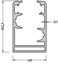
900-1101 (1,475 kg/mt) GOLD KASA PROFİLİ
