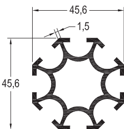
ST-3230 / 1,166 kg/mt
