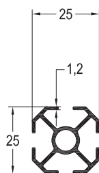
ST-313 / 0,399 kg/mt
