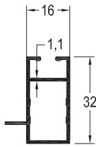
ST-121 / 0,334 kg/mt
