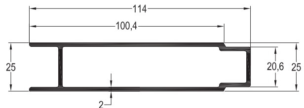
L-3080/20 / 1,475 kg/mt LAMBRI PROFİLİ
