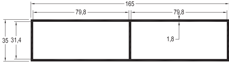
FS-4143 / 2,069 kg/mt MEKANİZMA KUTU PROFİLİ
