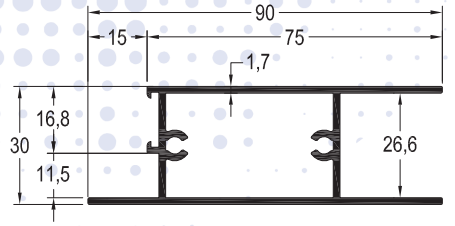
FS-4140 / 1,130 kg/mt ALT ETEK PROFİLİ
