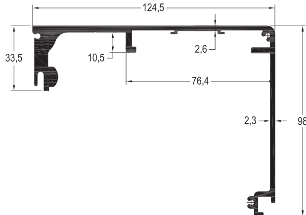
FS-4119 / 2,476 kg/mt ŞASE PROFİLİ
