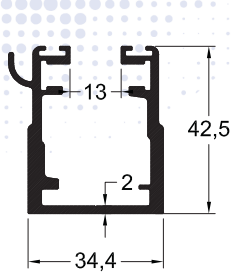
AS-1815 / 0,915 kg/mt KASA PROFİLİ
