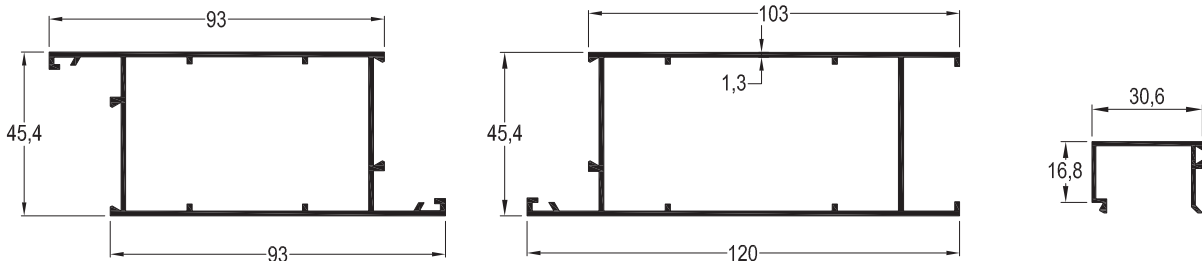
AL-3045 (1,088 kg/mt) KAPI KANAT PROFİLİ
